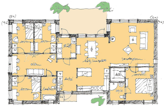
Bottenplan Boa = 147.2 m 2
